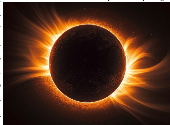
Solar Eclipse close-up image.
